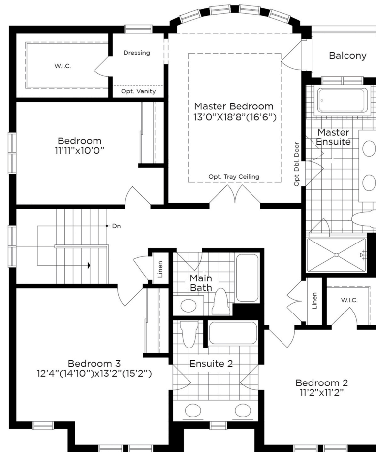
Second Floor
